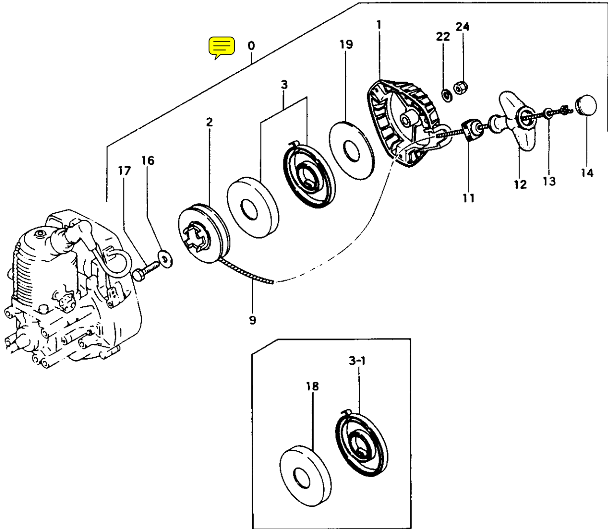
FIG.2 RECOIL STARTER
